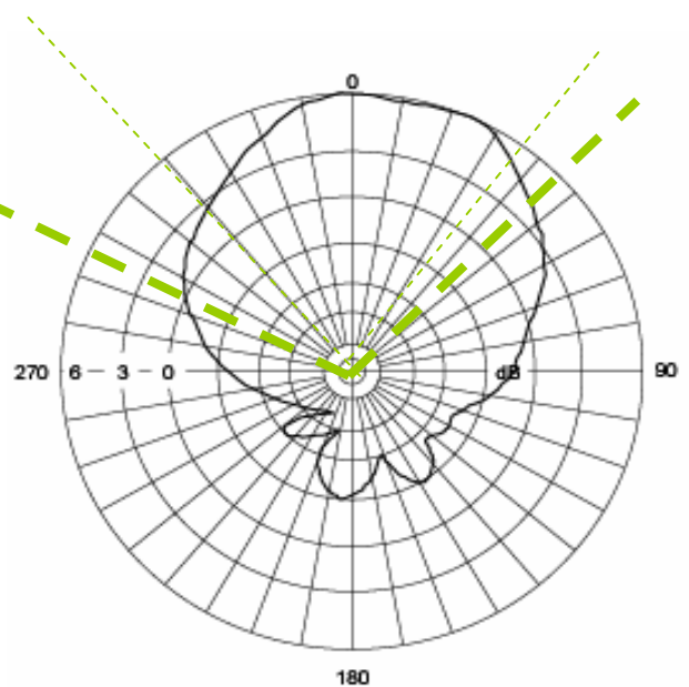
Vertical (E Plane)
