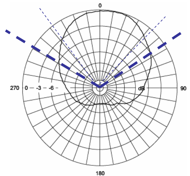
Horizontal (H Plane)
